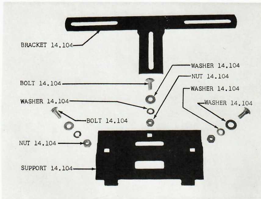
GROUP 14 - FIG. 1 - REAR LICENSE PLATE BRACKET 10-20-80 (WWC)
